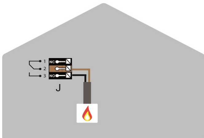
Potential-free switching contacts for additional functions
