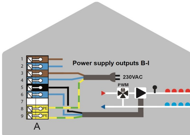
Mains connection heating circuit pump
