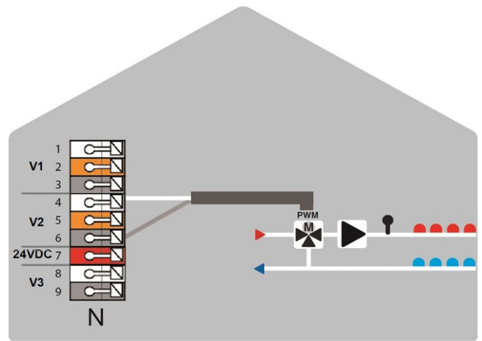
0-10V/PWM outputs for additional functions
